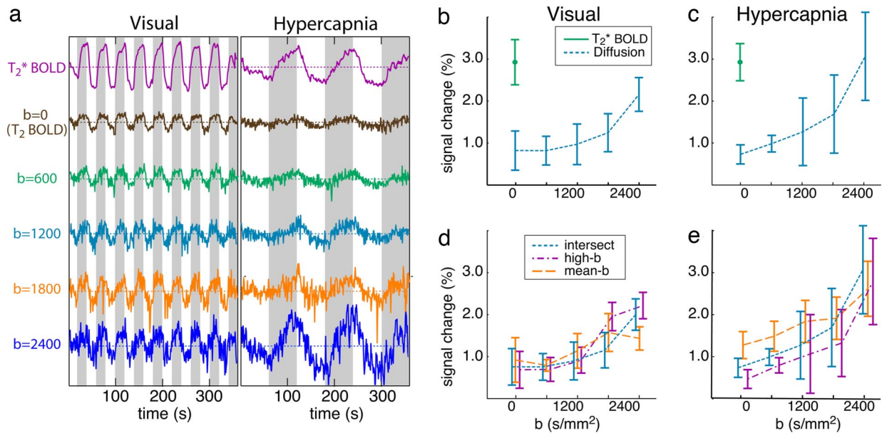
Fig. 1. Results from Experiments 1 (visual) and 2 (hypercapnia) combined across all subjects. (a) Mean subject time course within the “intersect” ROI for each imaging condition. Gray swathes indicate stimulation periods. All plots are scaled to the same percent signal change. (b–e) The percent signal as a function of b value, with each condition plotted as intersubject mean \pm intersubject standard deviation. (b and c) The percent signal change in the “intersect” ROI, including BOLD (green) and DFMRI (blue), over the range of acquired b values. (d and e) Percent signal change in the DFMRI data for the different ROI selection methods (plots are horizontally staggered to aid in visualization).
