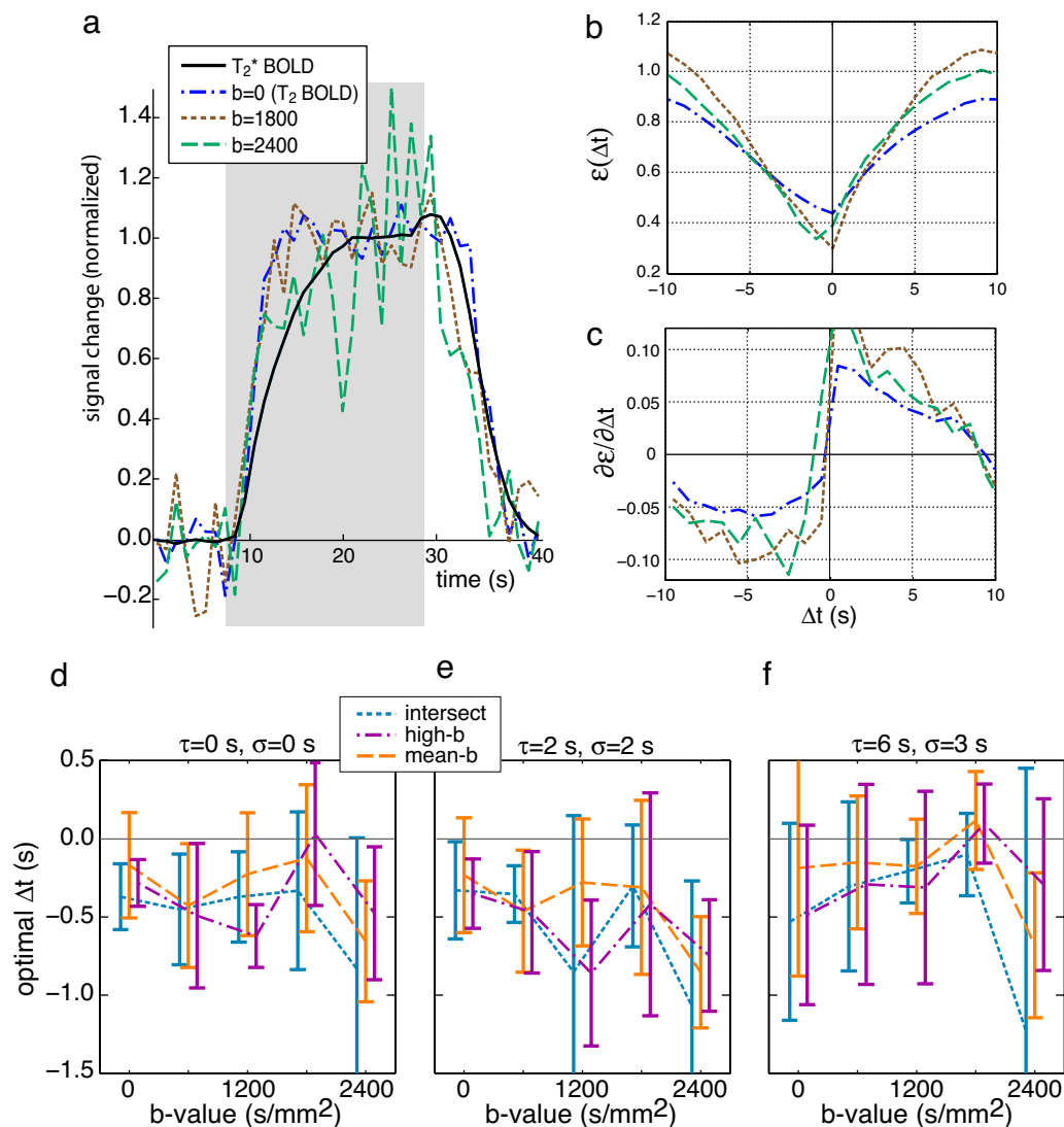
Fig. 2. Timing analysis for the visual experiment. (a) Intersubject mean response to a single block of visual stimulation. All time courses are normalized to unit plateau for timing analysis. The stimulus duration is noted by the gray swathe (the time courses have been shifted by 8 seconds for ease of display). (b) Normalized RMS error between T_2^* BOLD and time-shifted DFMRI time-courses. This error is minimized when the two curves are maximally aligned, and the shift ( \Delta t ) at which this occurs will be referred to as the “optimal time shift.” (c) Derivative of the normalized RMS error shown in b, which will cross zero at the optimal time shift. (d–f) The optimal time shift for the different ROI selection methods (“intersect,” “mean-b,” and “high-b”) and several signal models with slight changes in the expected timing of the signal (where \tau delays and \sigma smooths the time course). Previous work has reported an optimal time shift at high b value that is 2–4 seconds earlier than at low b value. No significant difference of this kind is observed in our data.
